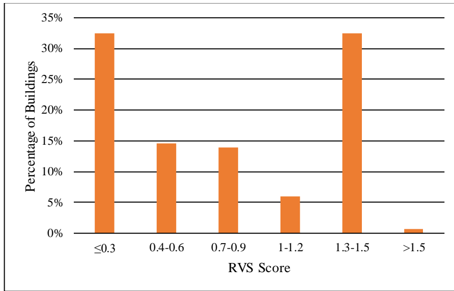
Figure 4.1 (a): Relations between percentage of buildings and RVS Score of Ward no 14 for moderately high seismicity
