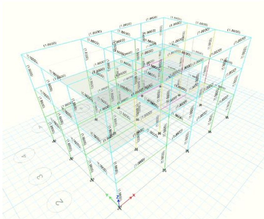
Figure 5.3: 3-D view of the building in FEM after analysis
