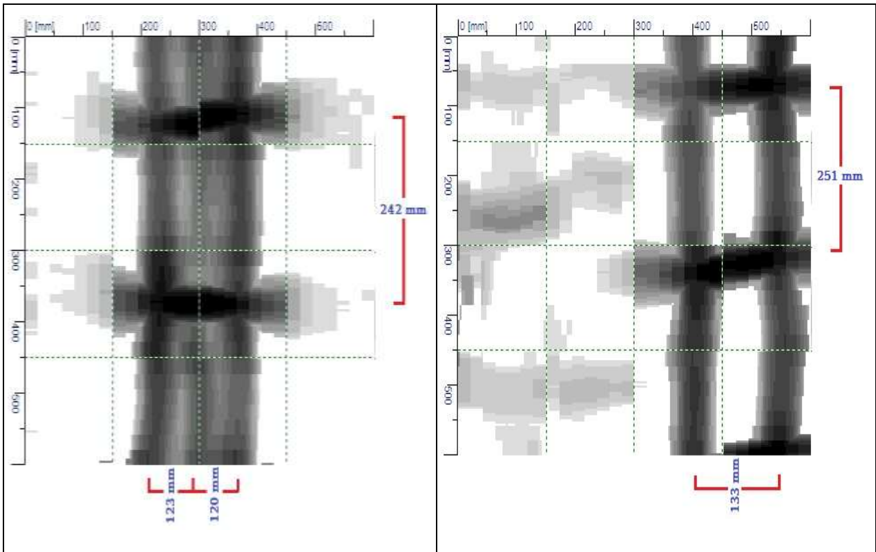
Figure E-01: Image scan of column GF-D5 (Long Side)
