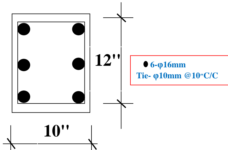
Figure E-03: Cross section of column GF-D5
