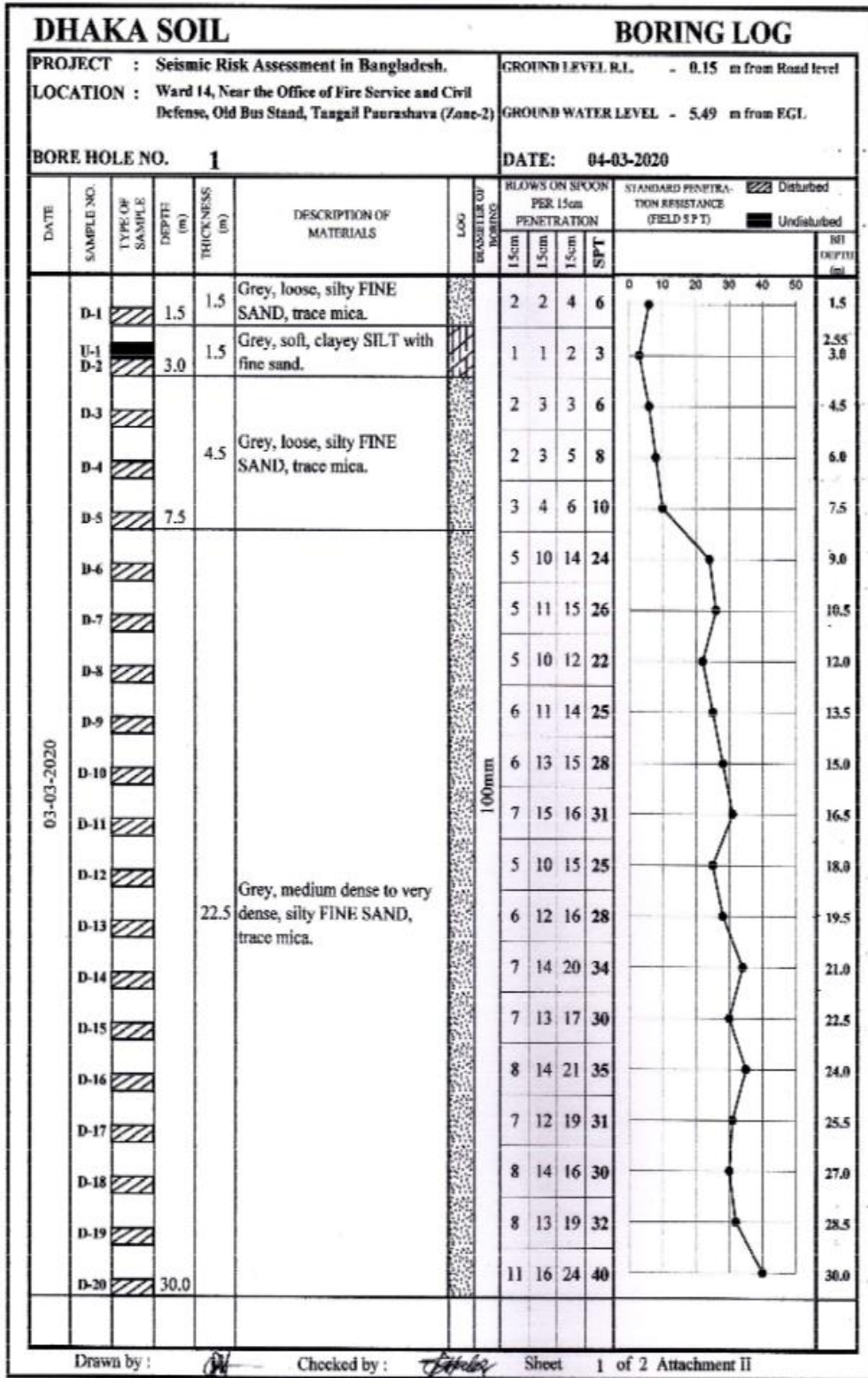
Figure 3.1: SPT data of Bore Hole 1 of Ward 14
