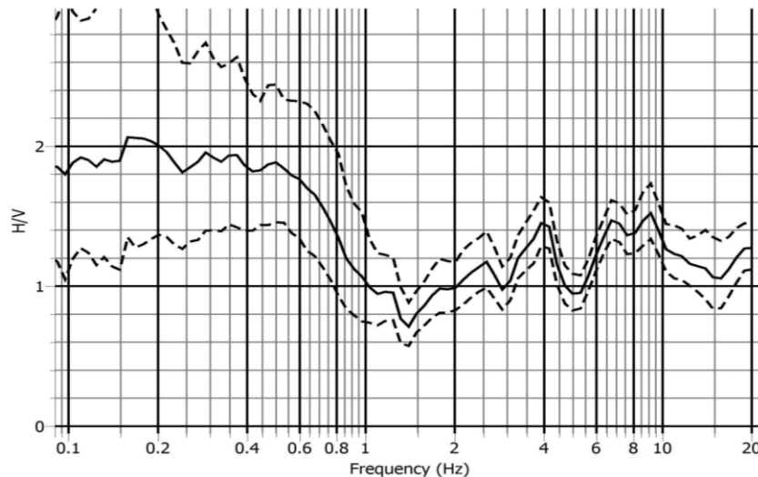
Figure 3.3: Amplitude vs Frequency graph of Ward no. 14 of Tangail Pourashava
