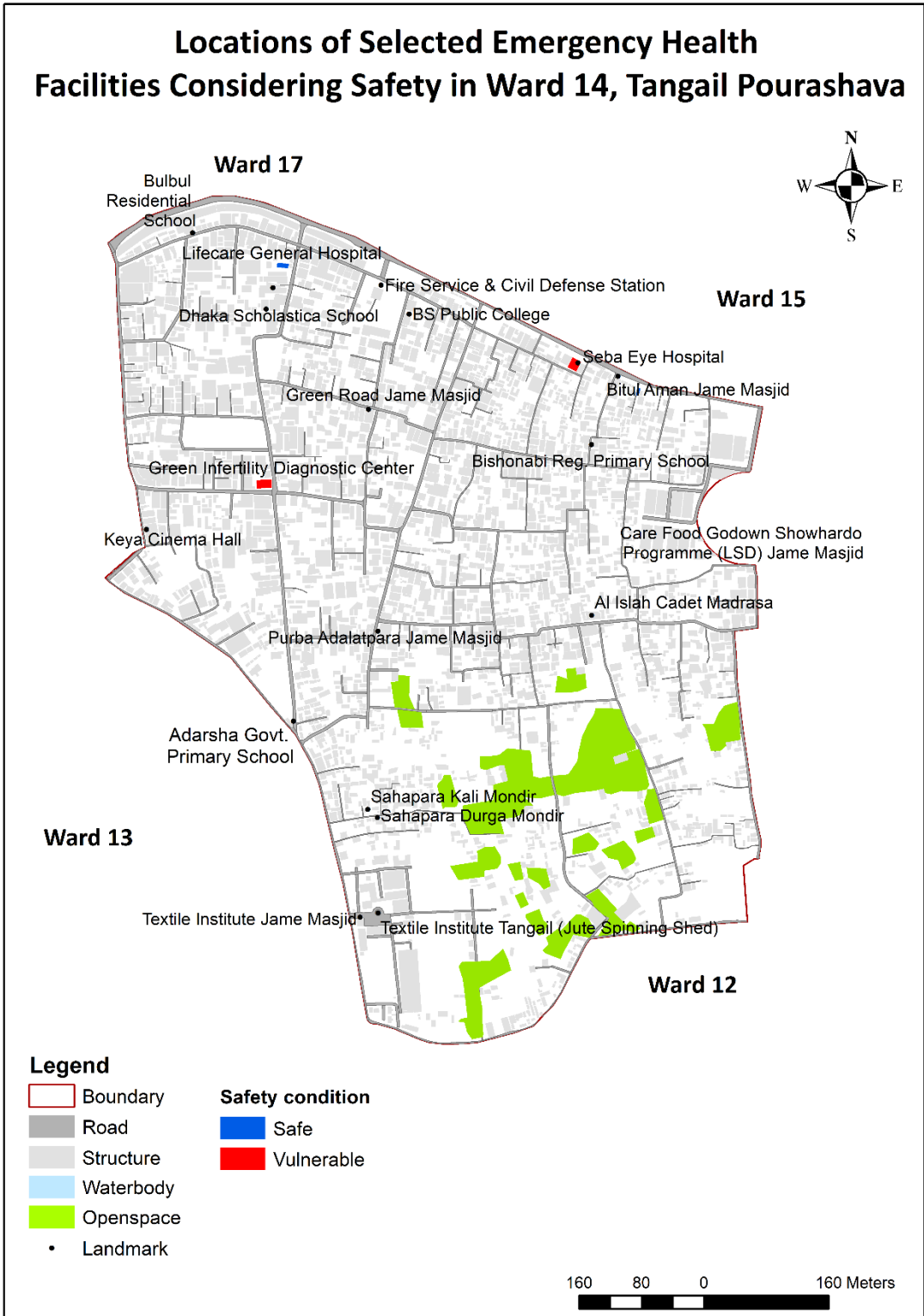
Figure 7.4: Location of selected emergency health facilities in the study area considering safety
