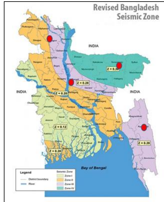
Figure 1.2: Revised Seismic Zoning of Bangladesh
