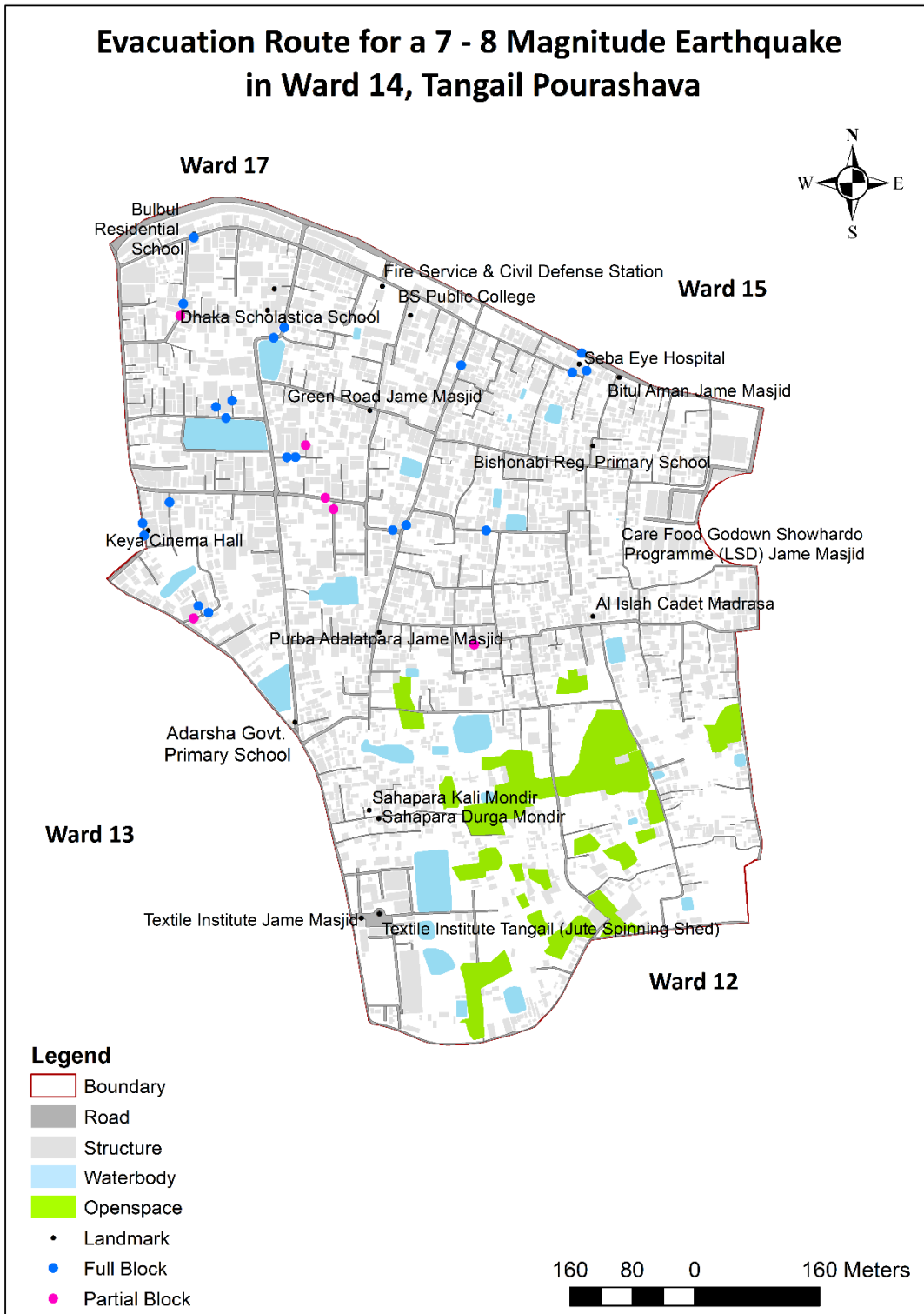
Figure 7.7: Evacuation Route for Scenario 01
