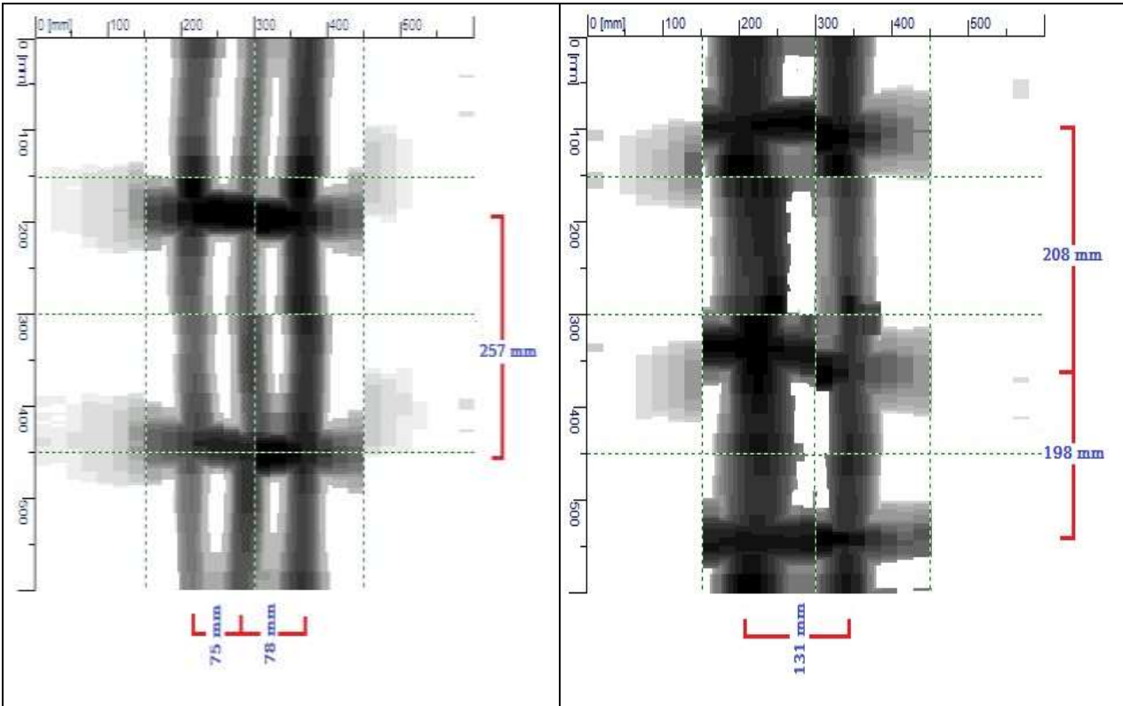
Figure E-04: Image scan of column GF-A5 (Long Side)
