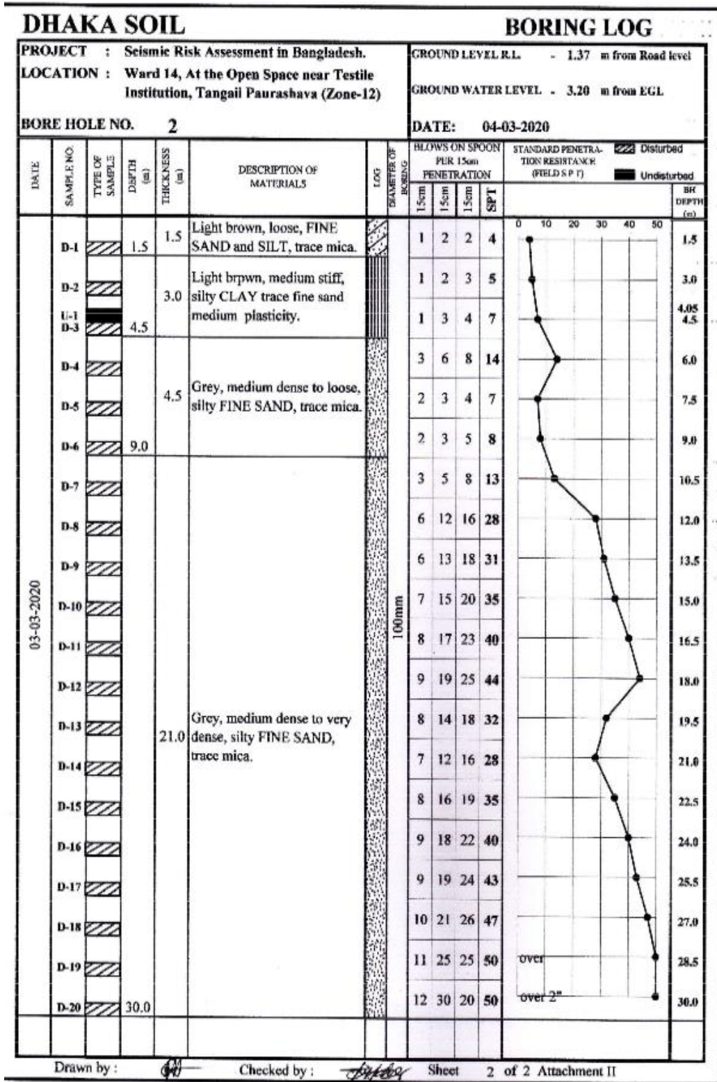
Figure 3.2: SPT data of Bore Hole 2 of Ward 14
