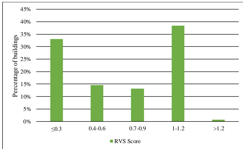
Figure 4.1 (b): Relations between percentage of buildings and RVS score of ward no 14 for high seismicity
