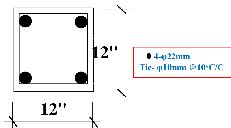
Figure E-13: Cross section of column GF-B2
