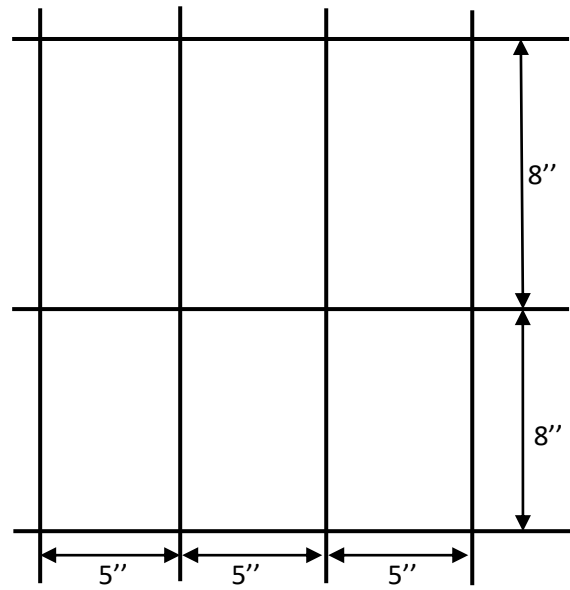
Figure E-21: Cross section of the slab 1F-S1
