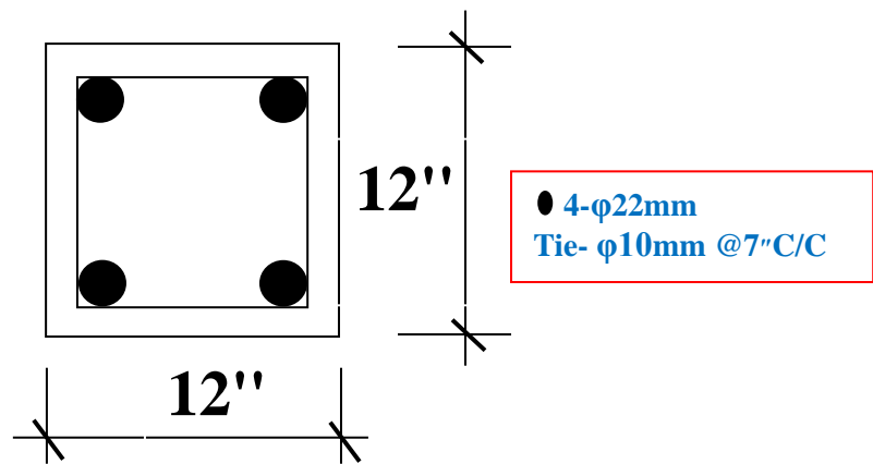
Figure E-16: Cross section of column 2F-B2
