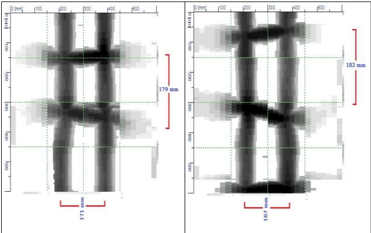
Figure E-08: Image scan of column GF-C1 (Long Side)
