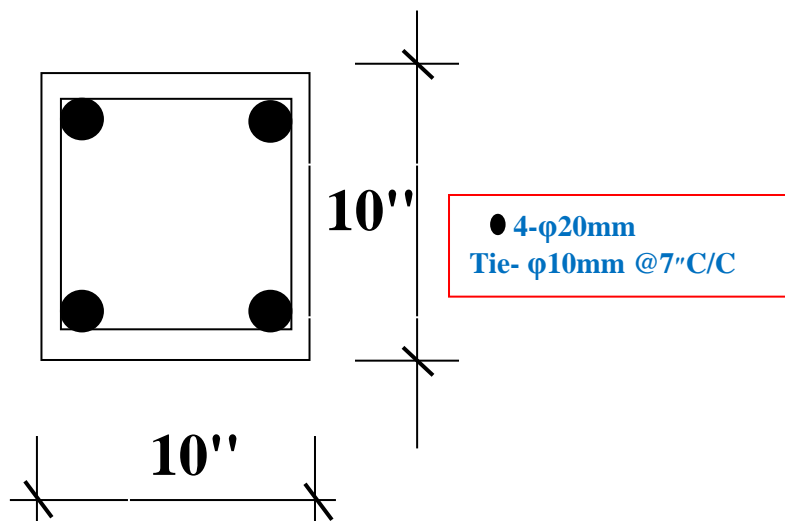
Figure E-10: Cross section of column GF-C1
