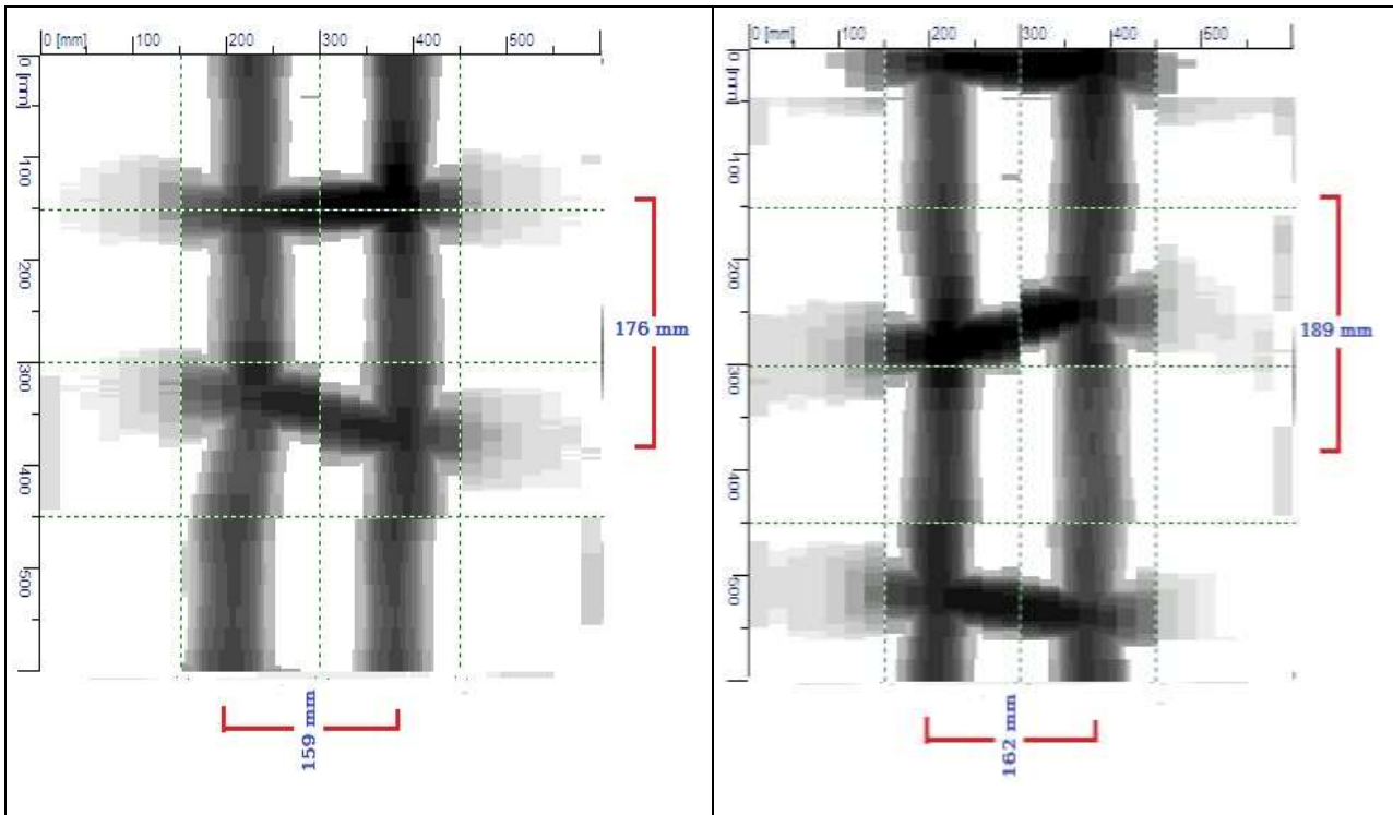
Figure E-14: Image scan of column 2F-B2 (Long Side)
