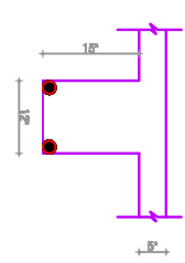
B-1 SECTION
