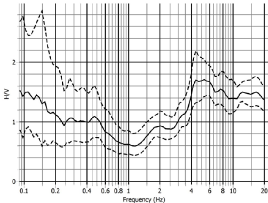
Figure 3.3: Amplitude Ratio vs Frequency graph of Ward no. 4 of Sunamganj Pourashava
