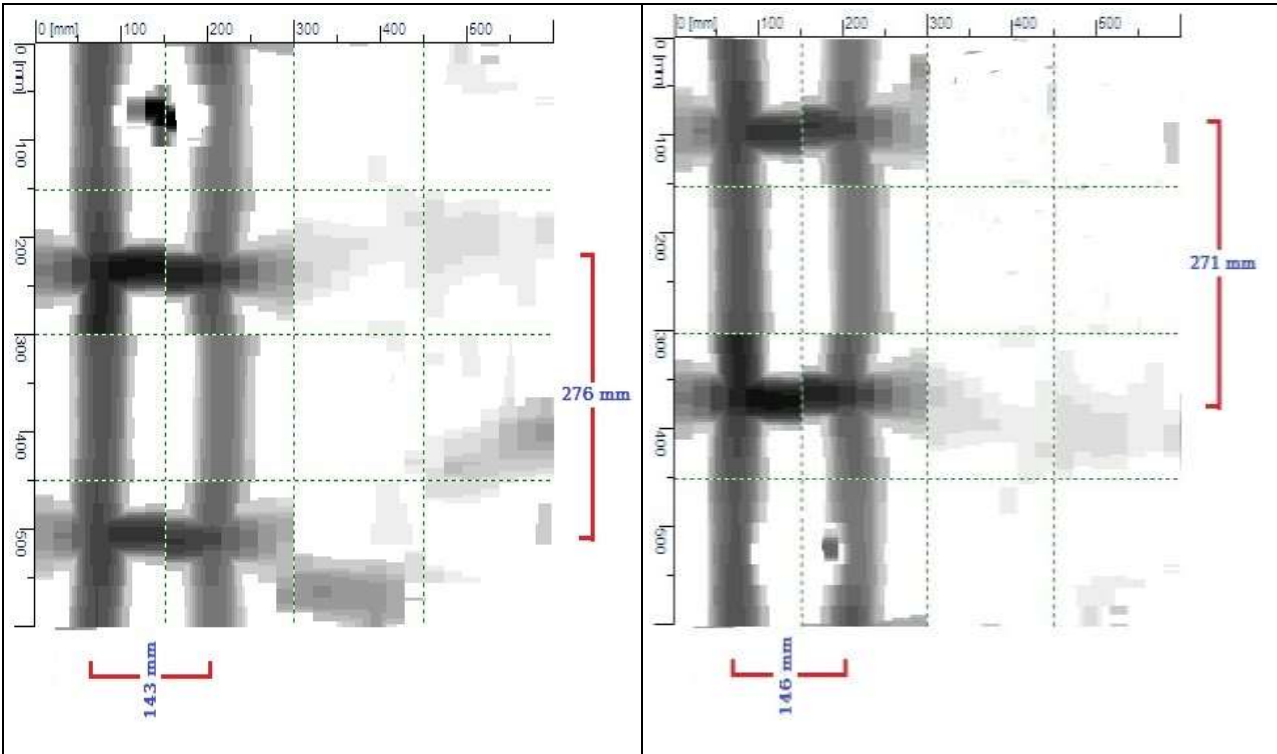
Figure E-01: Image scan of column GF-D4 (Long Side)
