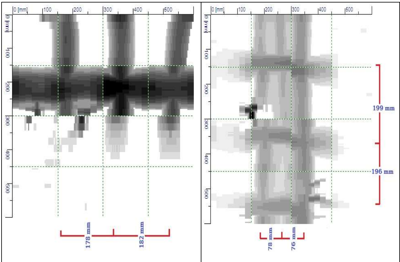
Figure E-10: Image scan of beam GF-B3 (lateral)
