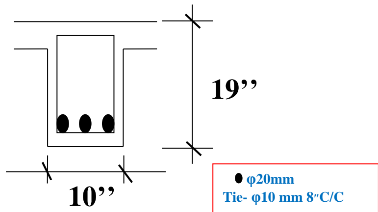
Figure E-12: Cross Section of Beam B3
