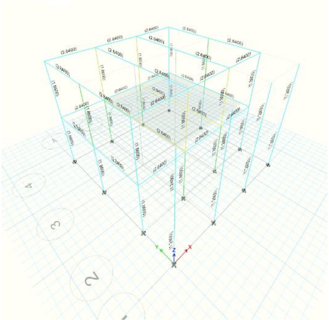
Figure 5.3: 3-D view of the building with reinforcement details after analysis
