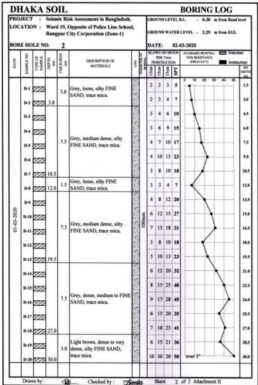
Figure 3.2: SPT data of Bore Hole 2 of Ward 19
