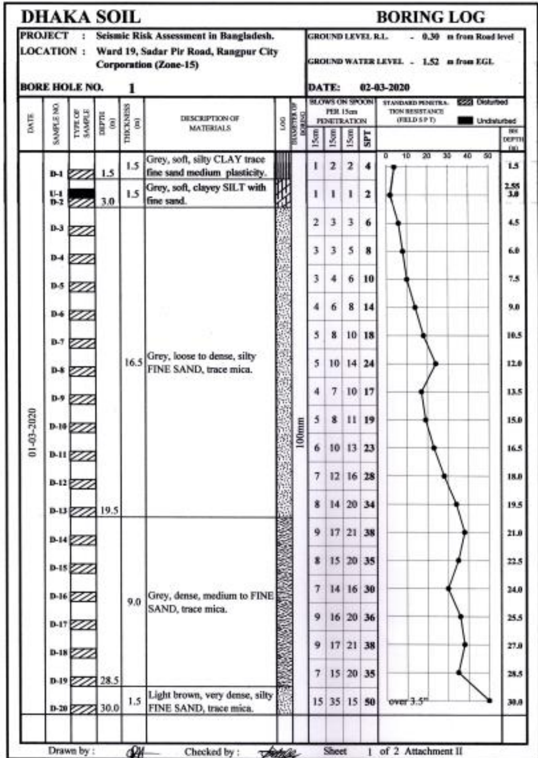
Figure 3.1: SPT data of Bore Hole 1 of Ward 19
