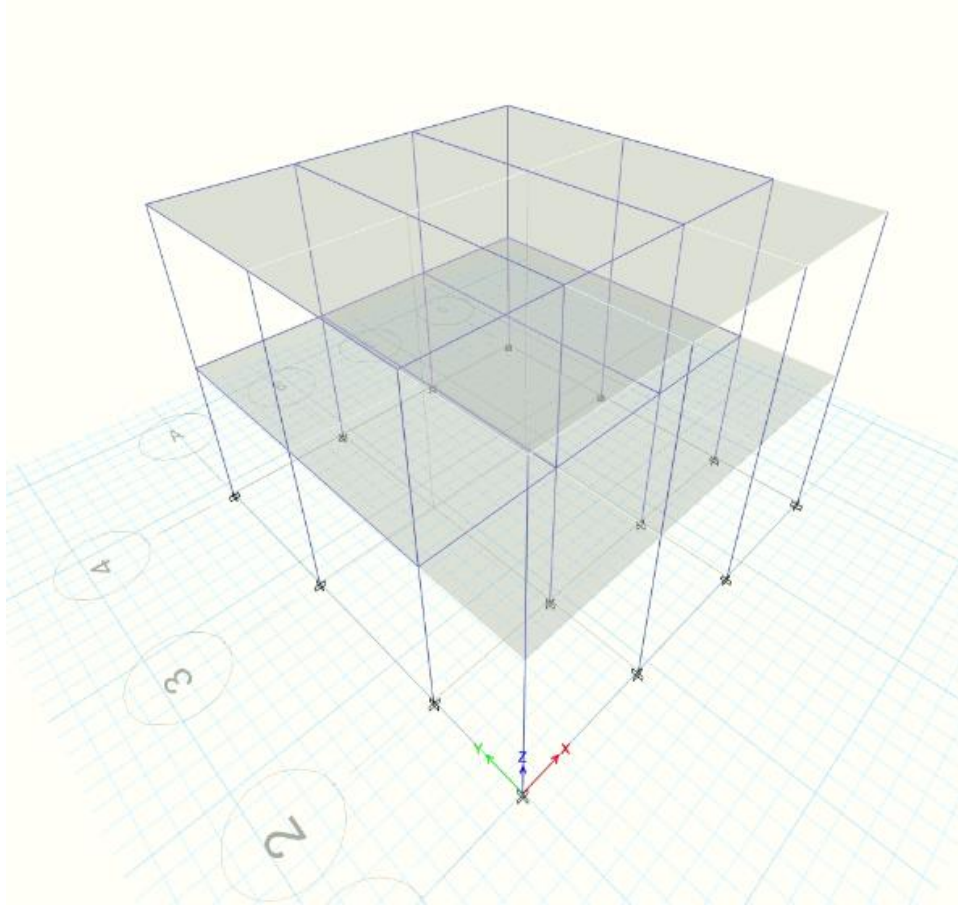
Figure 5.2: 3-D view of the finite element model before analysis
