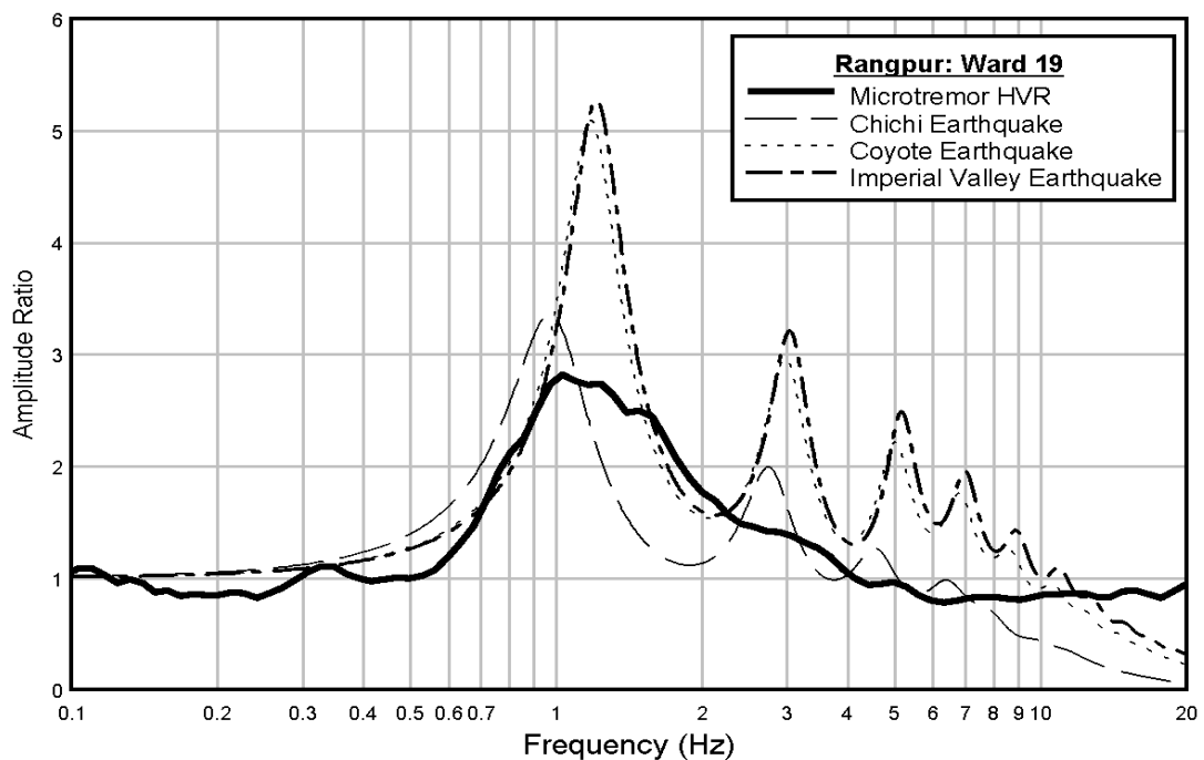
Figure 3.3: Amplitude vs Frequency graph of Ward no. 19 of Rangpur City Corporation
