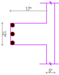
section of B-1
