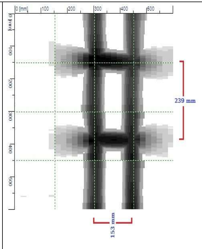
Figure E-05: Image scan of column GF-C1 (Short Side)
