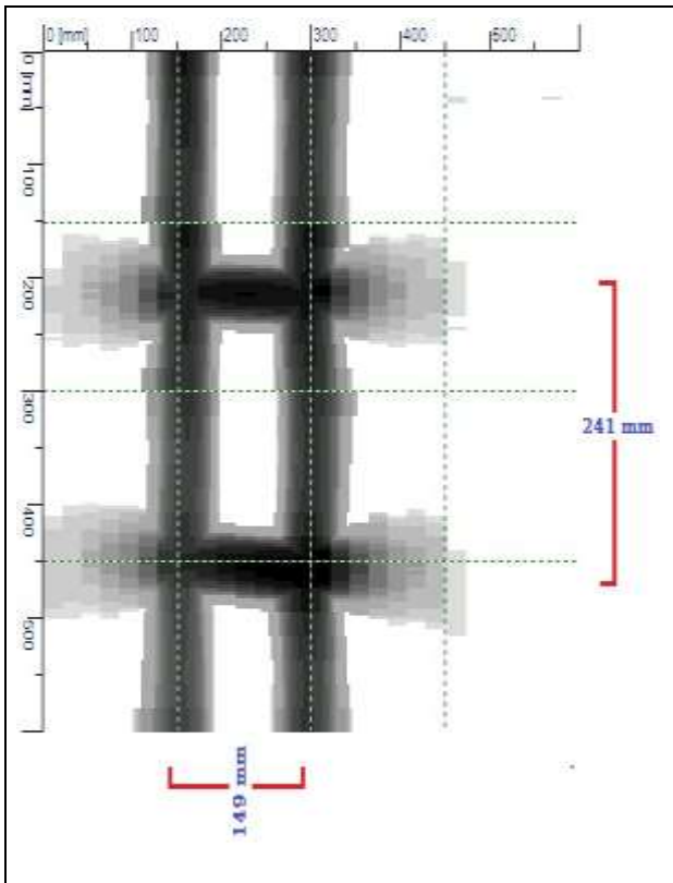
Figure E-04: Image scan of column GF-C1 (Long Side)
