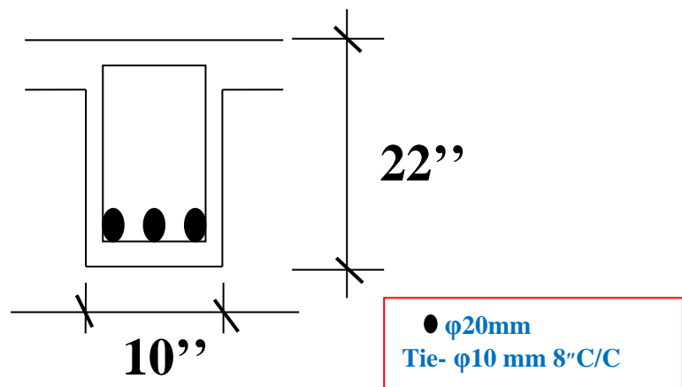
Figure E-09: Cross Section of Beam B1
