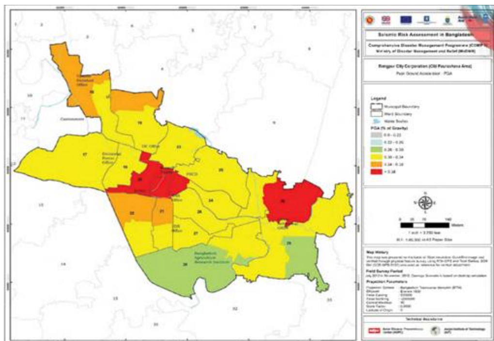
Figure 1.3: Peak Ground Acceleration map (Source: CDMP, 2015)
