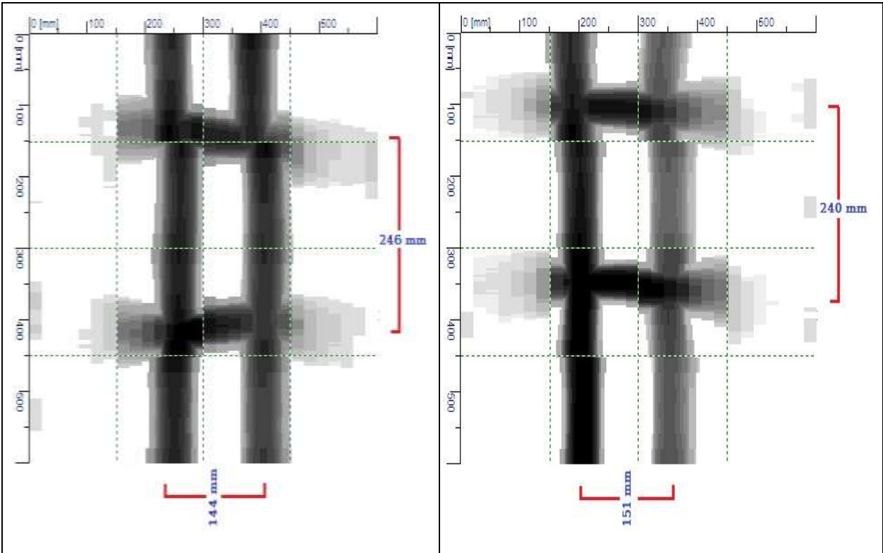
Figure E-01: Image scan of column GF-C1 (Long Side)
