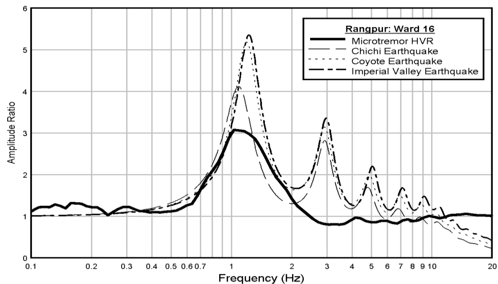
Figure 3.3: Amplitude Ratio vs Frequency graph of Ward no. 16 of Rangpur City Corporation
