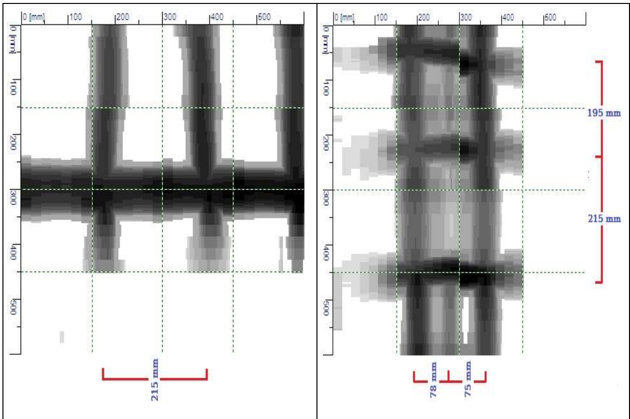
Figure E-07: Image scan of beam GF-B1 (lateral)
