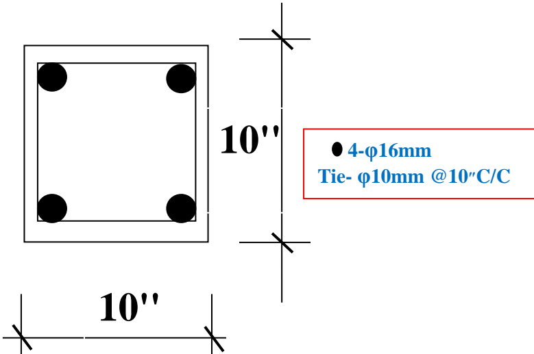
Figure E-03: Cross section of column GF-C1
