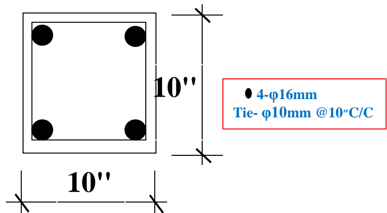
Figure E-06: Cross section of column GF-C1
